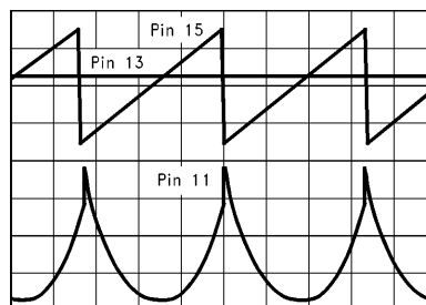
FIGURE 6. Raster Position Up
