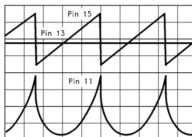
FIGURE 7. Raster Position Down
