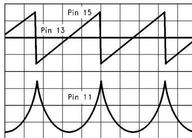
FIGURE 5. Raster Position Centered
